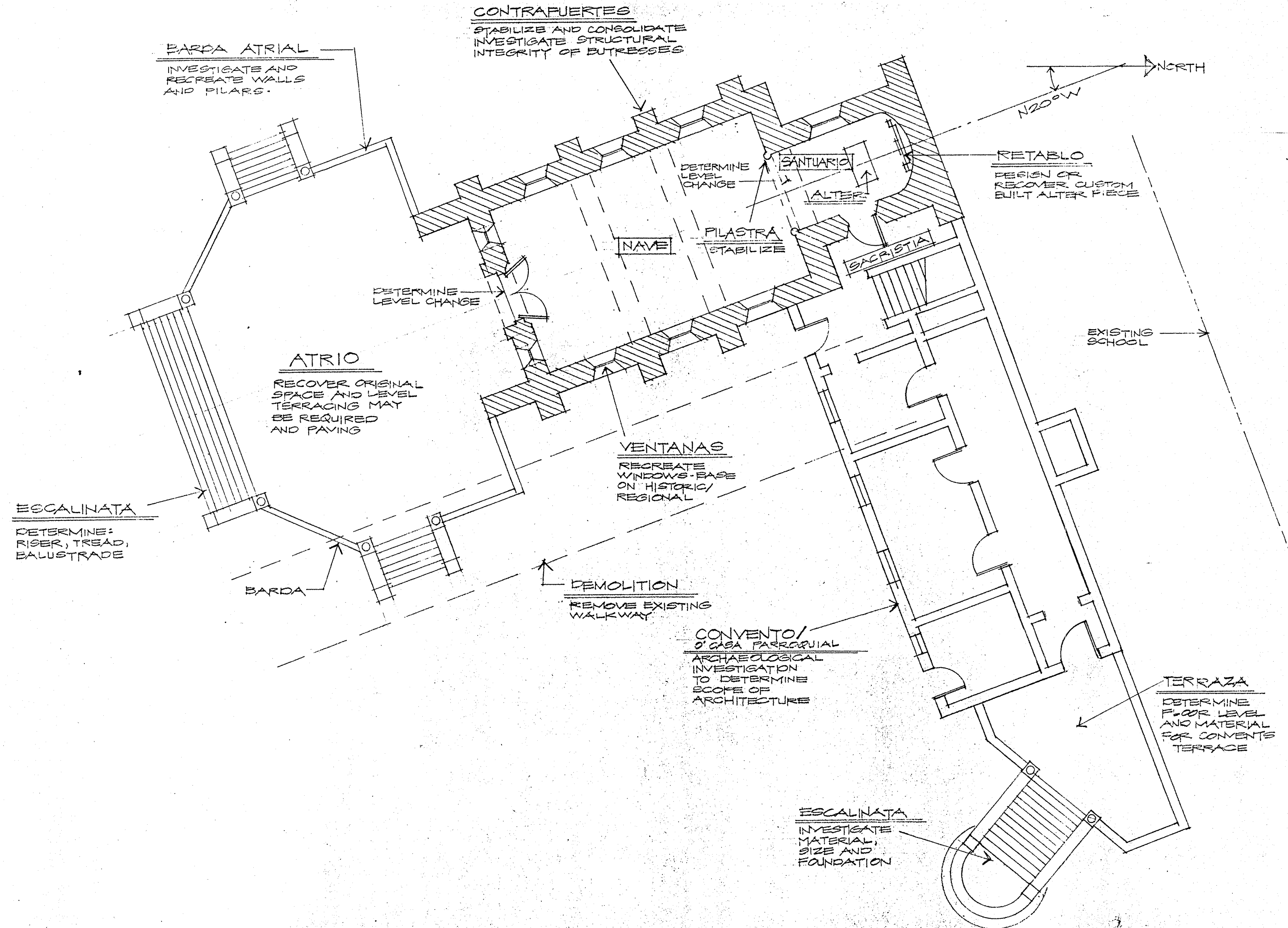
← NORTH FLOOR PLAN IGLESIA de NUESTRO SEÑOR de SAN DIONICIO NTS BASED ON: SURVEY BY DUPRENEY ON THE 1816 FREYCENET EXPEDITION, AND FIELD OBSERVATION
